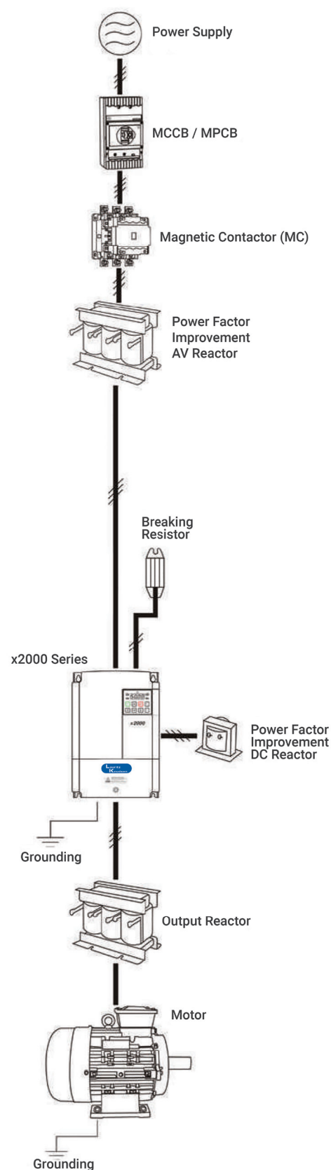
Connection Scheme
